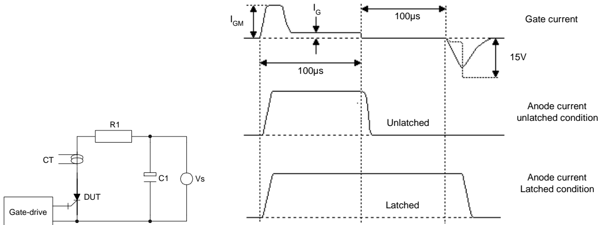
Diagram 4, Latching test circuit and waveforms.
