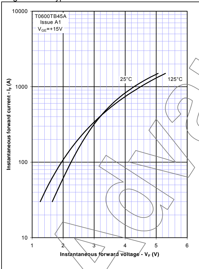
Figure 11 – Typical diode forward characteristic
