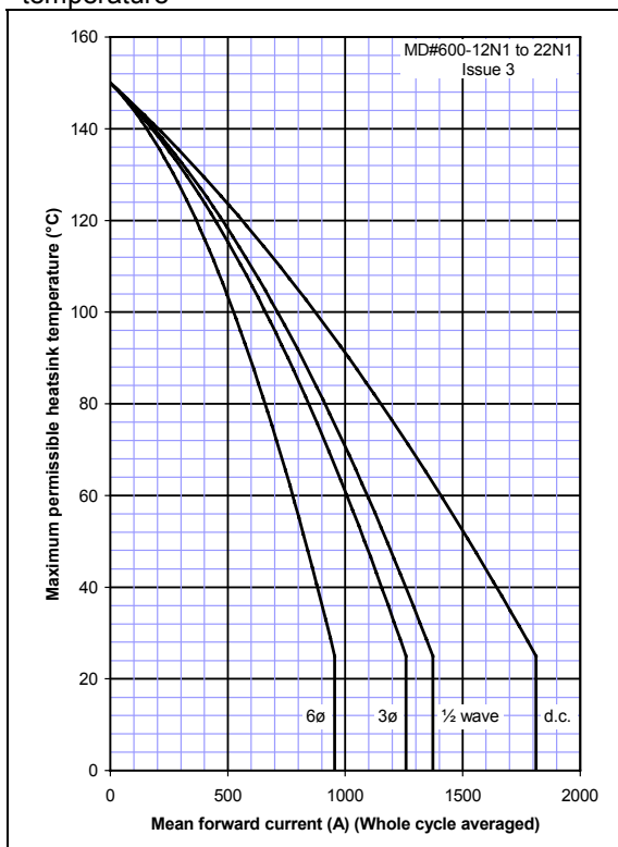
Figure 8 – Forward current vs. Heatsink temperature
